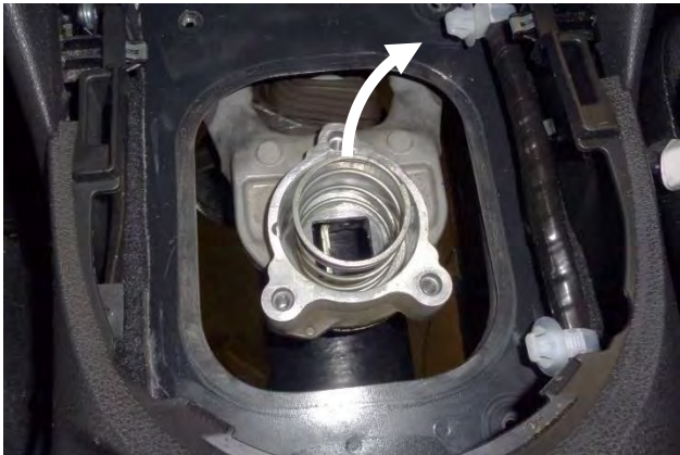
18. Remove and retain the spring.
