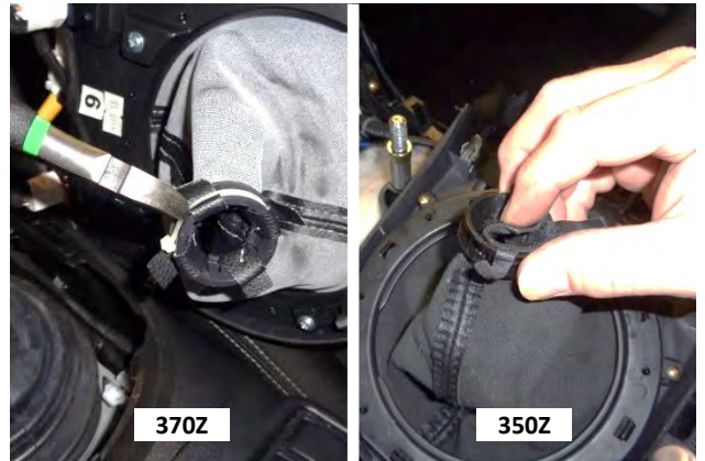
9. Remove the plastic ring from the leather boot. Some models (370Z and similar) require cutting a cable tie. Use care to avoid tearing the leather.
