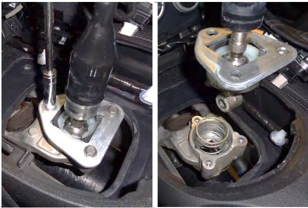
17. CAUTION: SHIFTER PLATE IS UNDER SPRING TENSION. Carefully remove the 3 shifter plate screws, then remove the shifter and plate. Retain the shifter plate for re-use.
