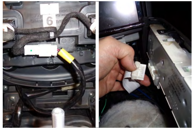
8. Disconnect all electrical connectors, and remove the shifter panel from the vehicle.
