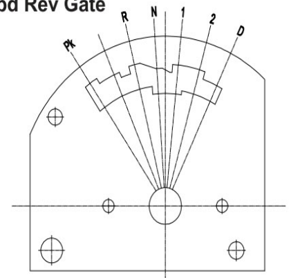
3 Spd Rev Gate
