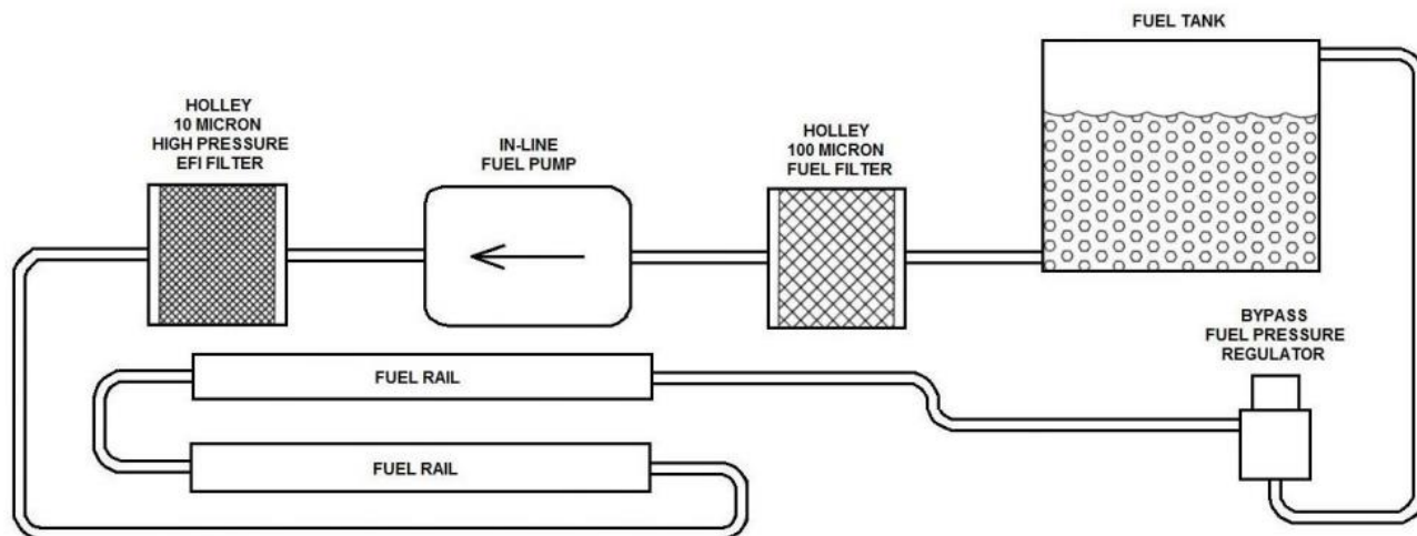
Plumbing Diagram
