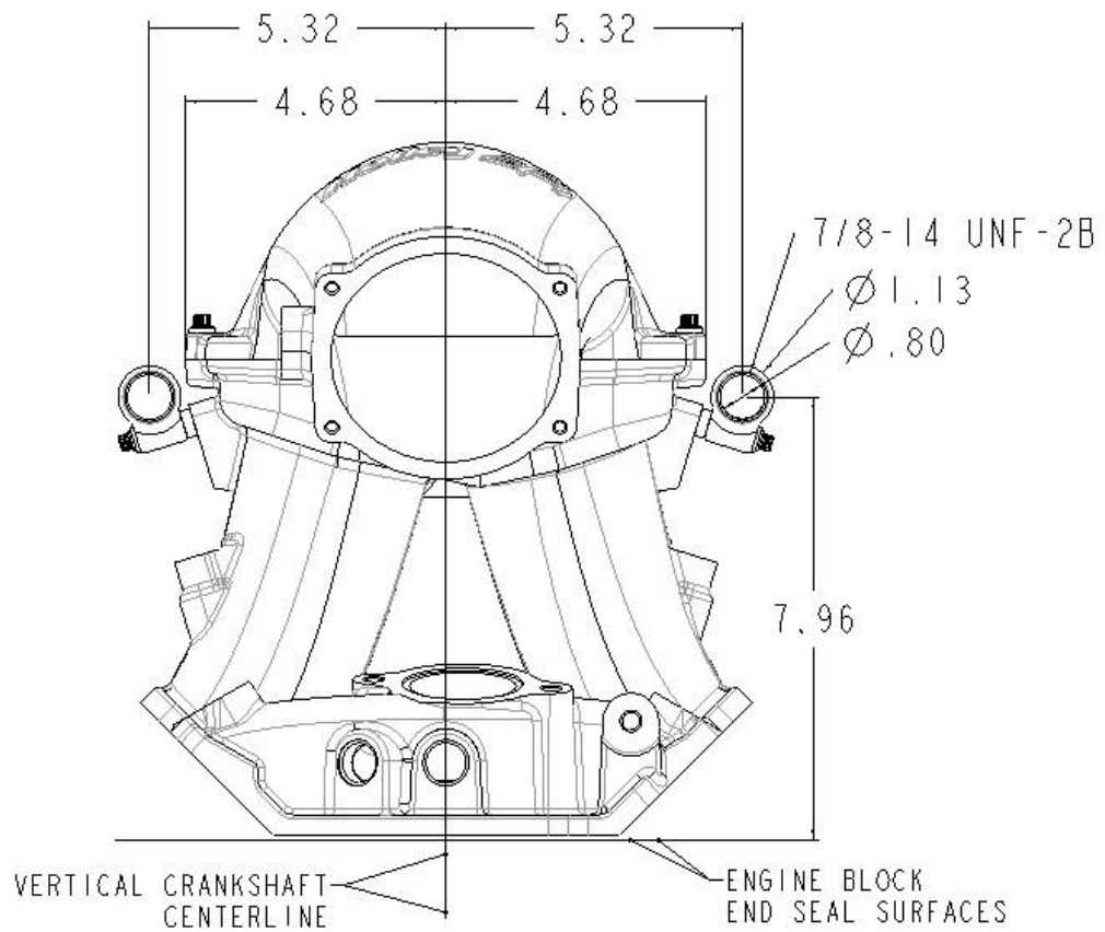
OUTLINE DIMENSIONS - 300-963
