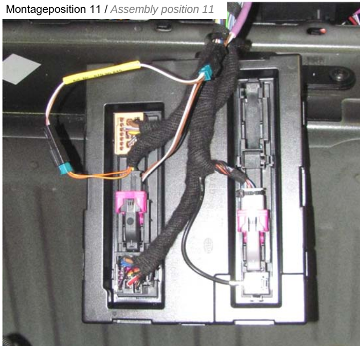
Montageposition 11 / Assembly position 11
