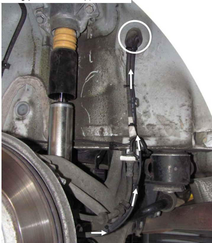
Montageposition 4 / Assembly position 4
