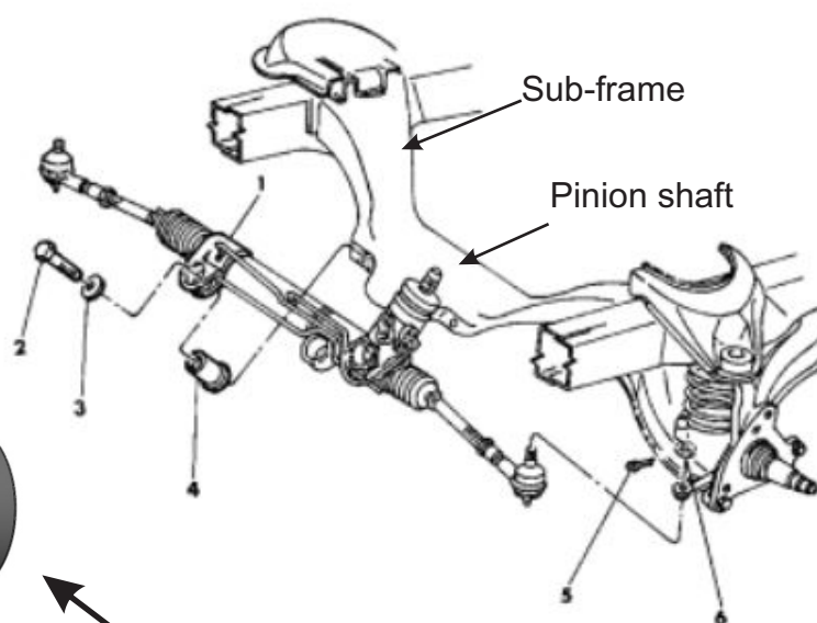
Bushing 91887 - rear
