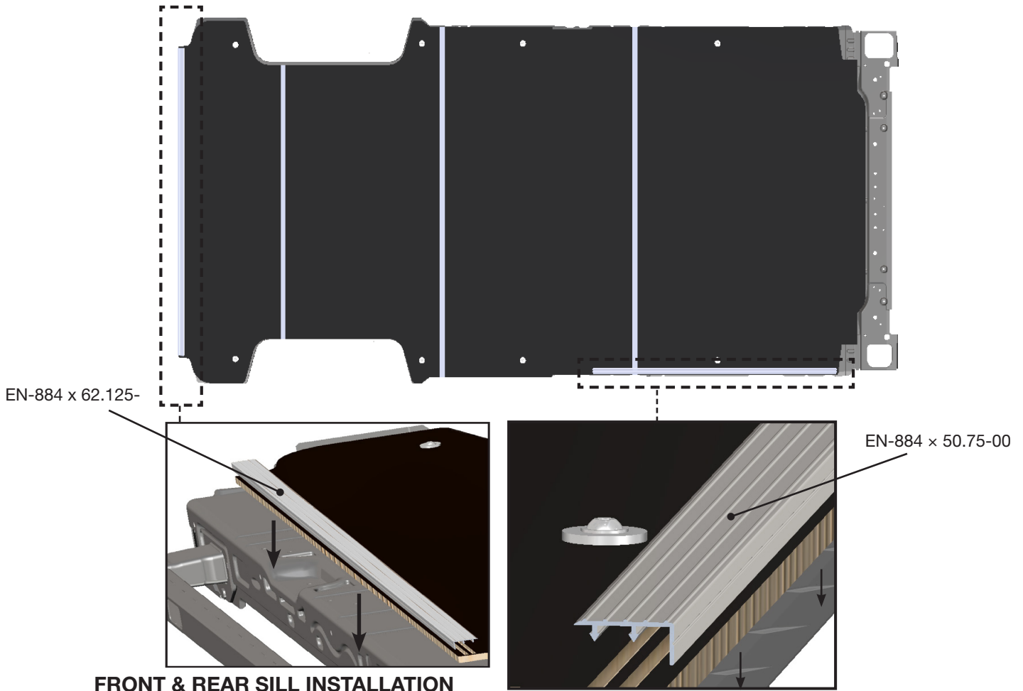
FRONT & REAR SILL INSTALLATION
